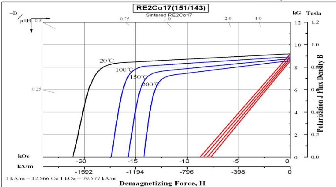
Demagnetization Curves
